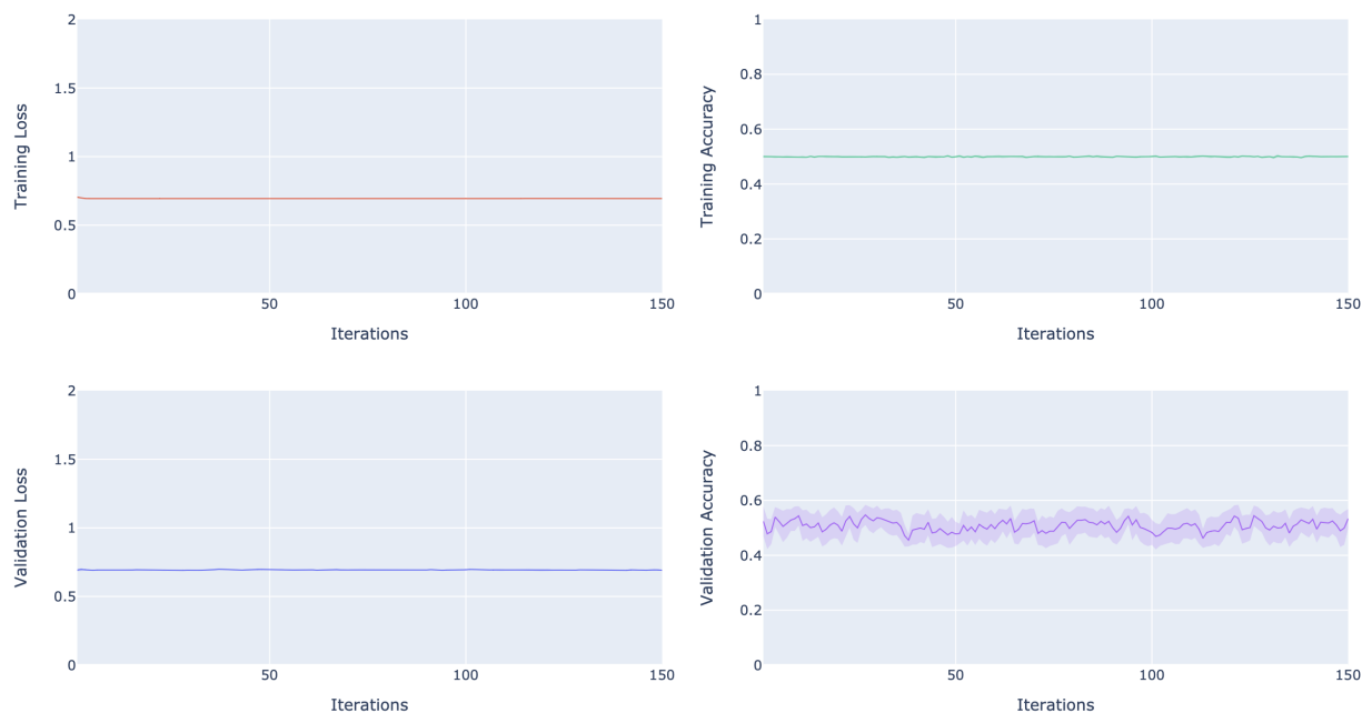
Figure 22: Alpha 1 - experiment 2 dataset A, 10 runs, CPU
