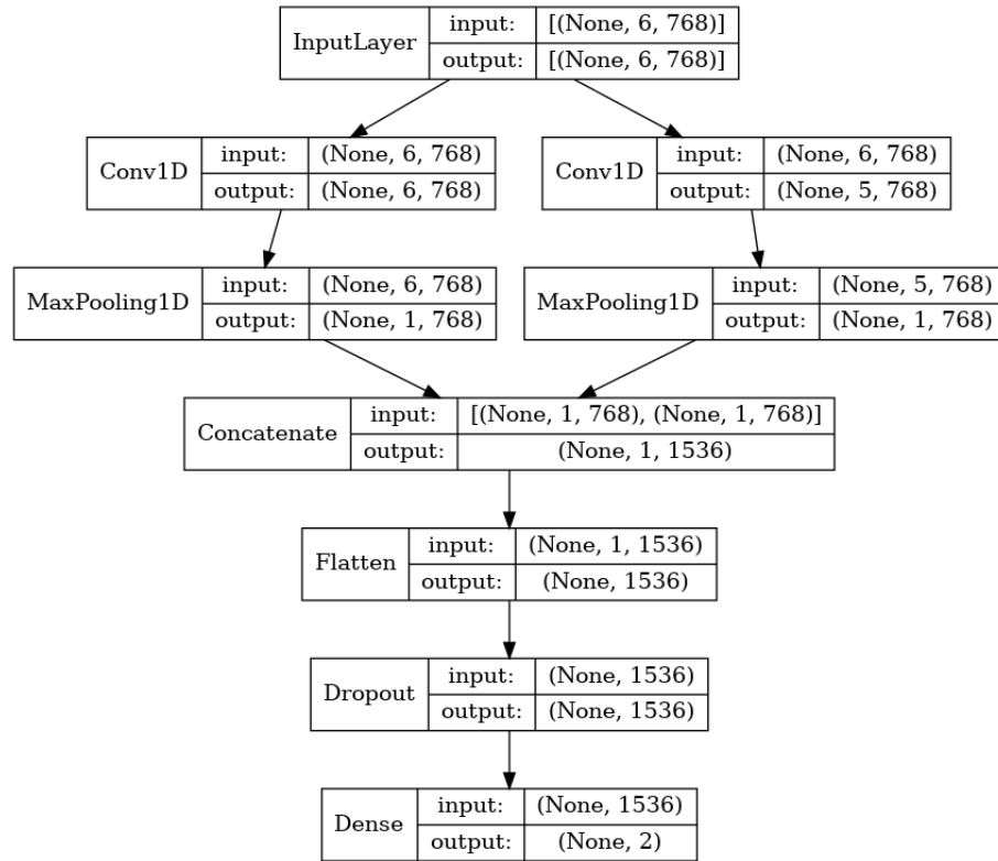
Figure 12: The architecture of the convolutional neural network
