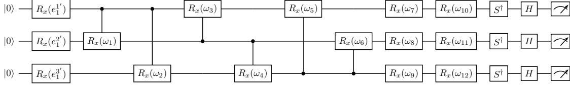
Figure 9: Quantum circuit favouring expressivity with n_{qubit} = 3 (Sim et al., 2019)
