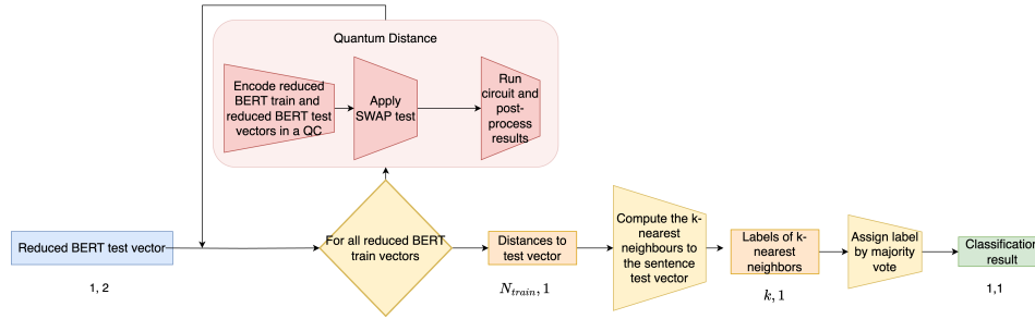
Figure 10: Beta 1 pipeline
