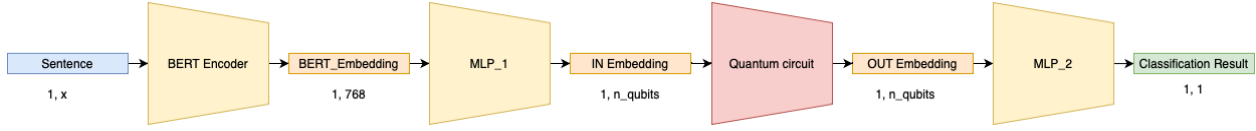
Figure 8: Alpha 3 pipeline
