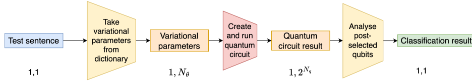
Figure 3: Pre-Alpha 1 pipeline
