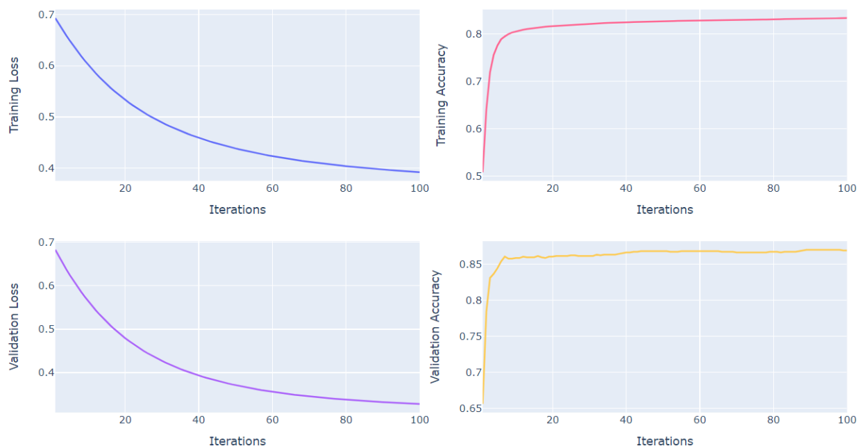
Figure 30: Shallow feed-forward neural network with Transformer sentence embeddings
