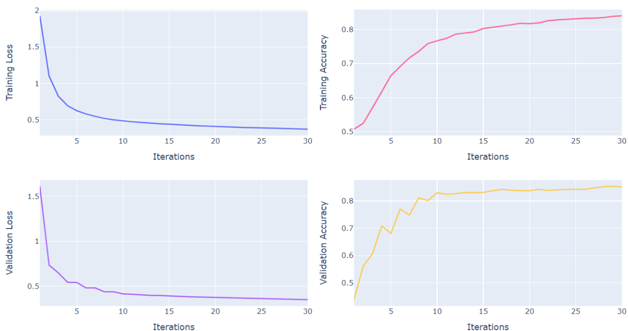
Figure 32: Convolutional network with BERT word embeddings
