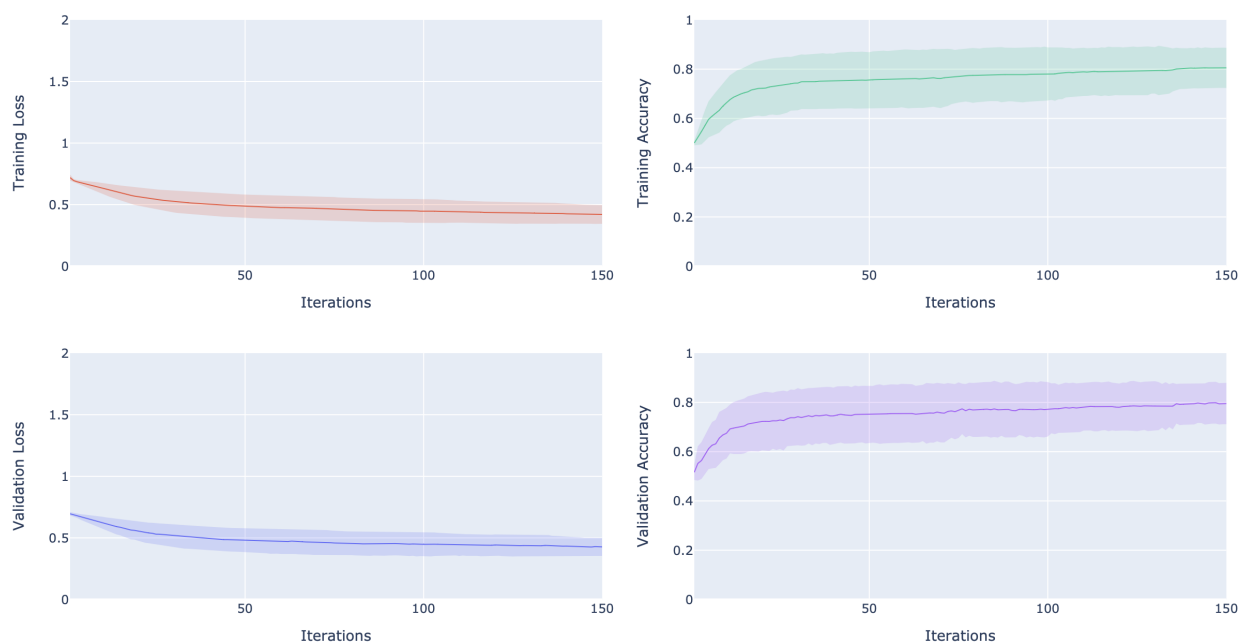
Figure 18: Alpha 3 - experiment 1 dataset B, 30 runs, CPU
