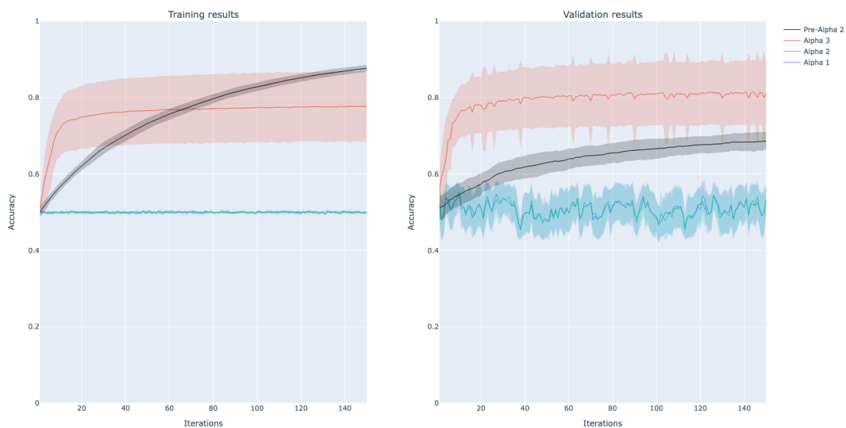
Figure 26: All model accuracies - experiment 2 dataset A, 10 runs, CPU
