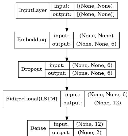
Figure 13: The architecture of the bidirectional LSTM neural network
