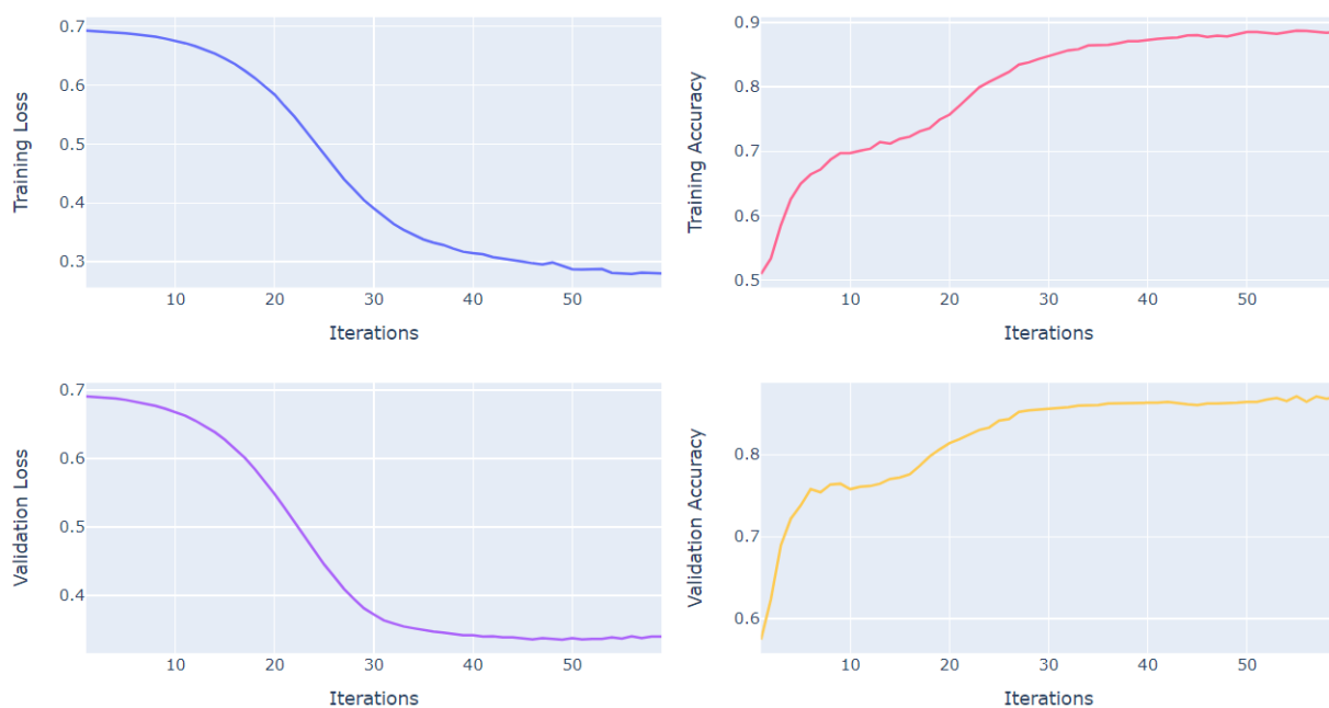
Figure 33: Bidirectional LSTM network without pre-trained embeddings
