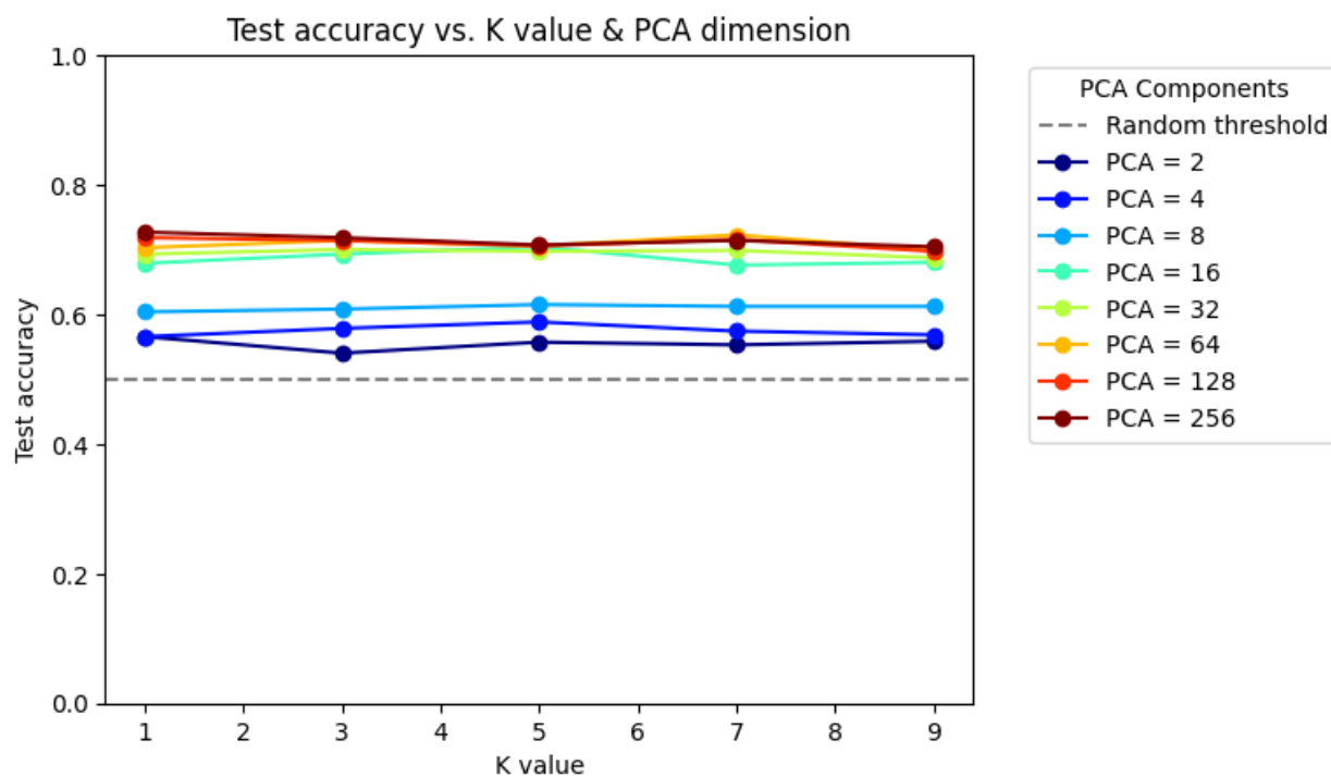
Figure 37: KNN experiment Dataset B dataset B, 1 run, CPU
