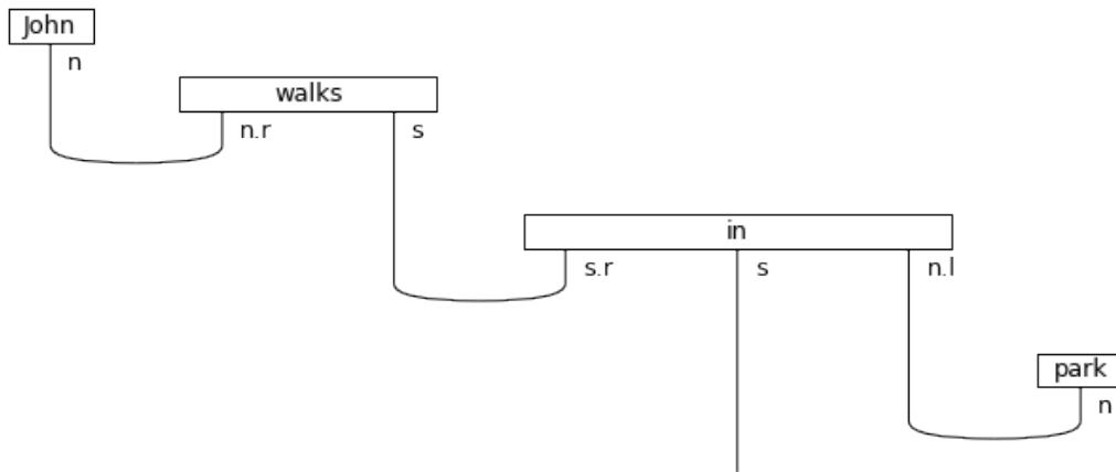
Figure 35: DisCoCat rewritten string diagram
