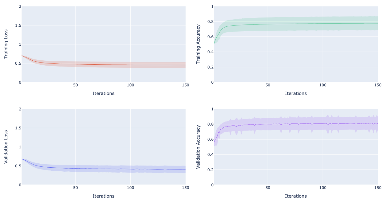
Figure 24: Alpha 3 - experiment 2 dataset A, 10 runs, CPU
