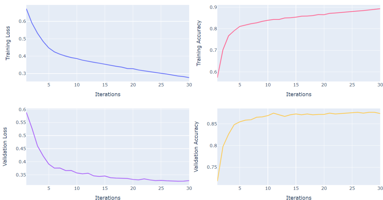
Figure 29: Convolutional network with FastText word embeddings
