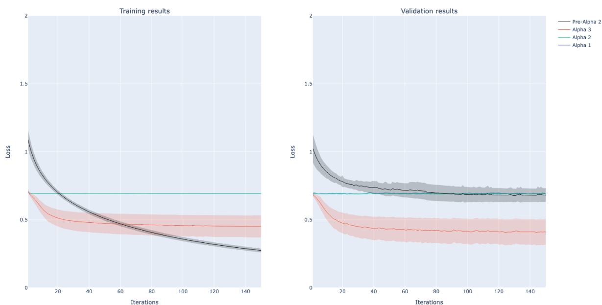
Figure 25: All model losses - experiment 2 2 dataset A, 10 runs, CPU
