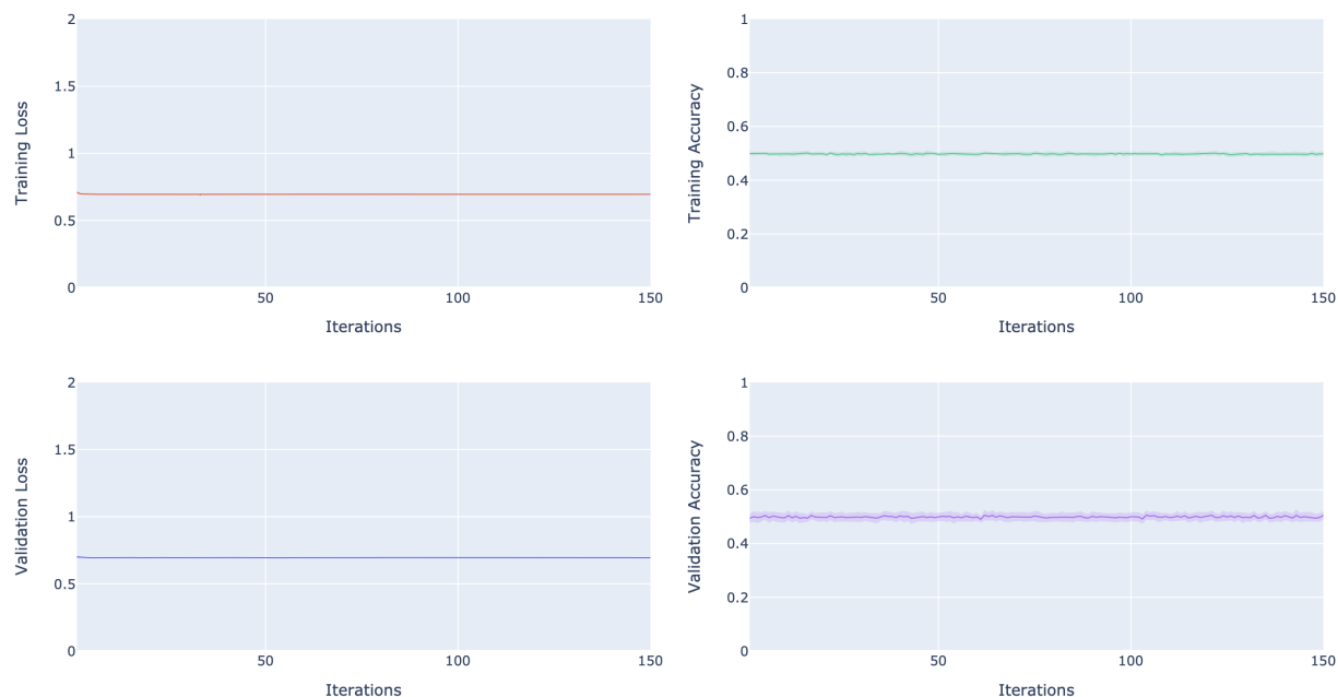
Figure 16: Alpha 1 - experiment 1 dataset B, 30 runs, CPU
