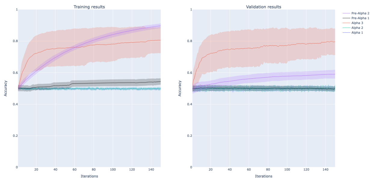
Figure 20: All model accuracies - experiment 1 dataset B, 30 runs, CPU
