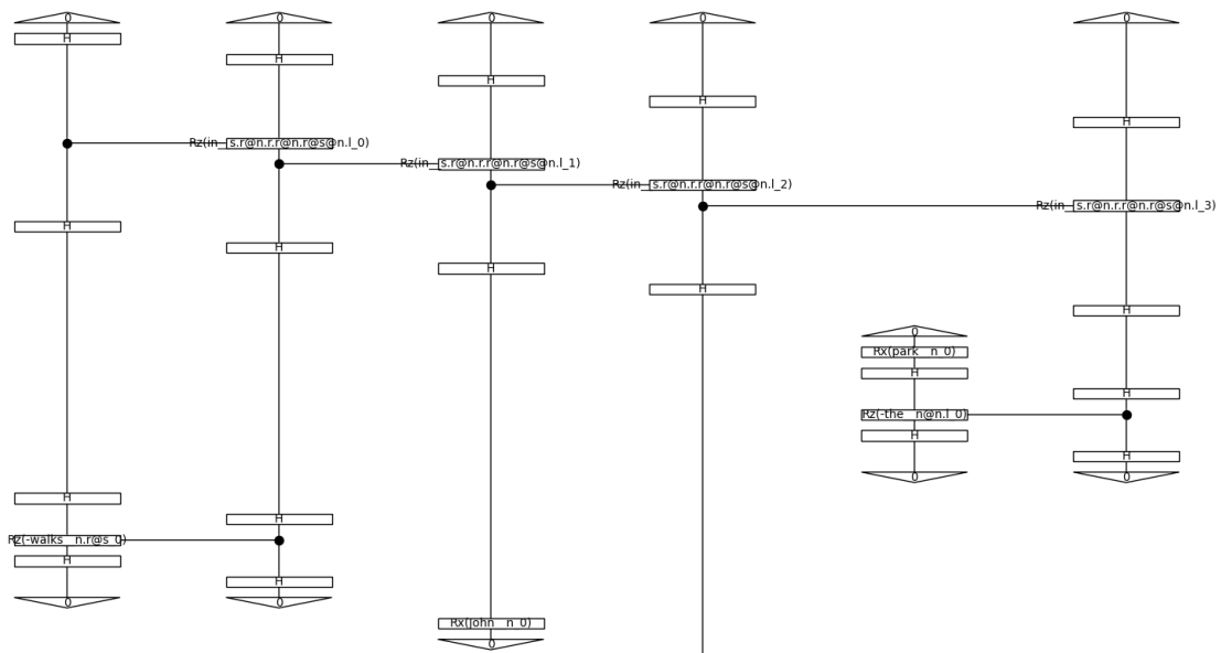
Figure 36: DisCoCat quantum circuit
