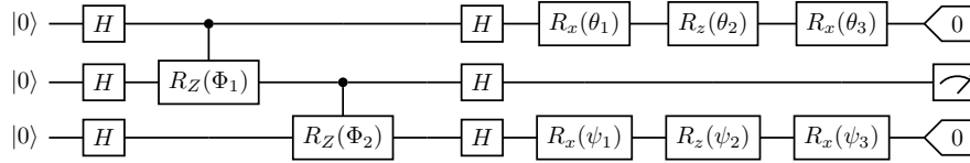
Figure 4: A choice of pre-Alpha 2 variational quantum circuit for the sentence “John likes Mary”
