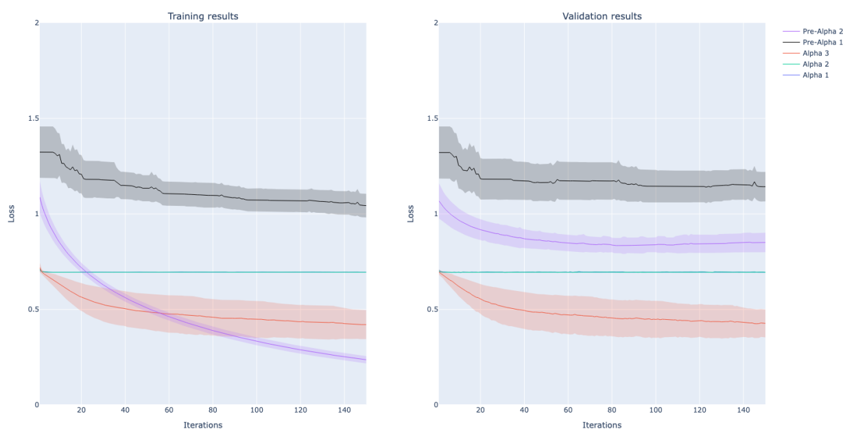
Figure 19: All model losses - experiment 1 1 dataset B, 30 runs, CPU
