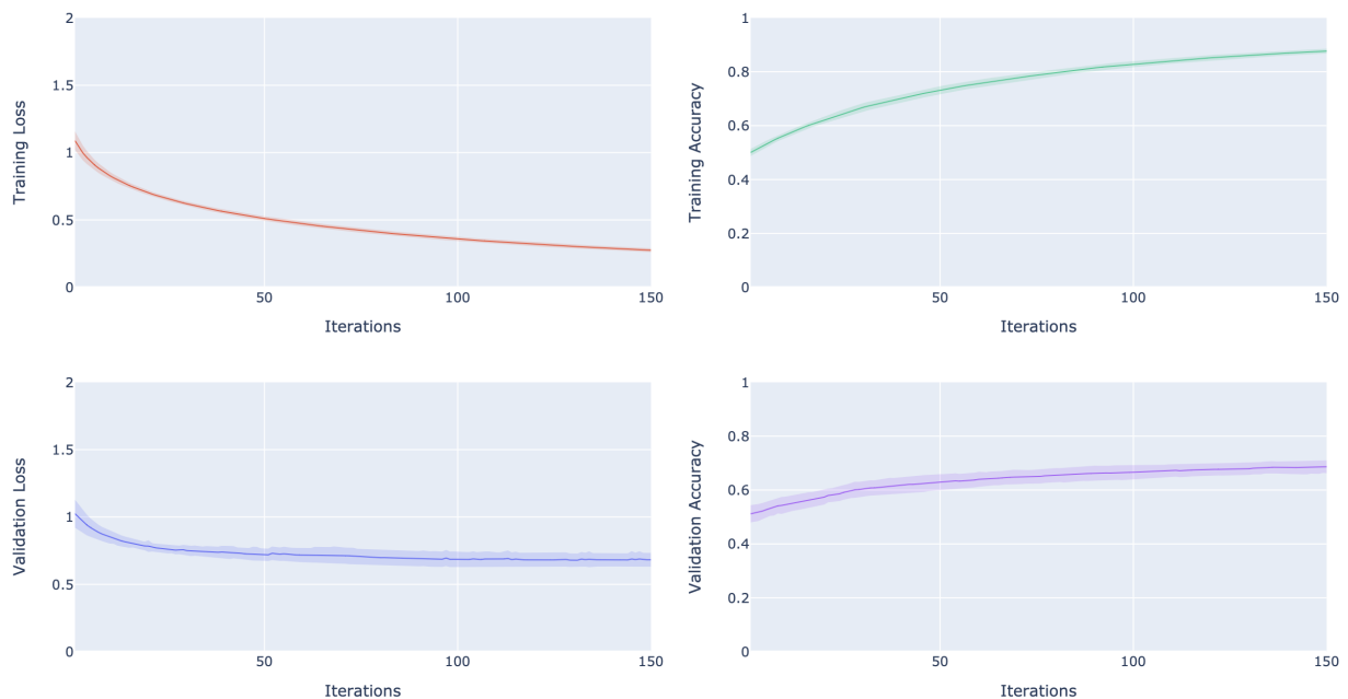
Figure 21: Pre-Alpha 2 train/validation loss and accuracy dataset A, 10 runs, CPU
