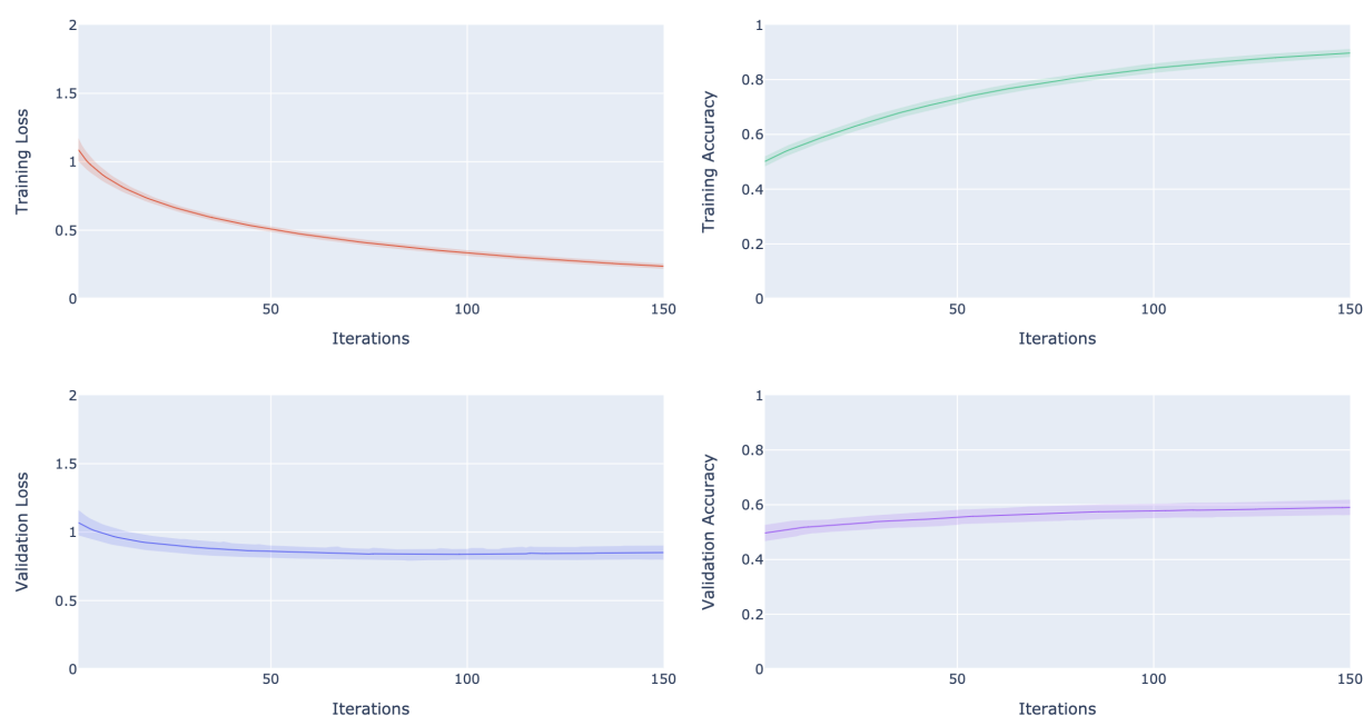
Figure 15: Pre-Alpha 2 - experiment 1 dataset B, 30 runs, CPU
