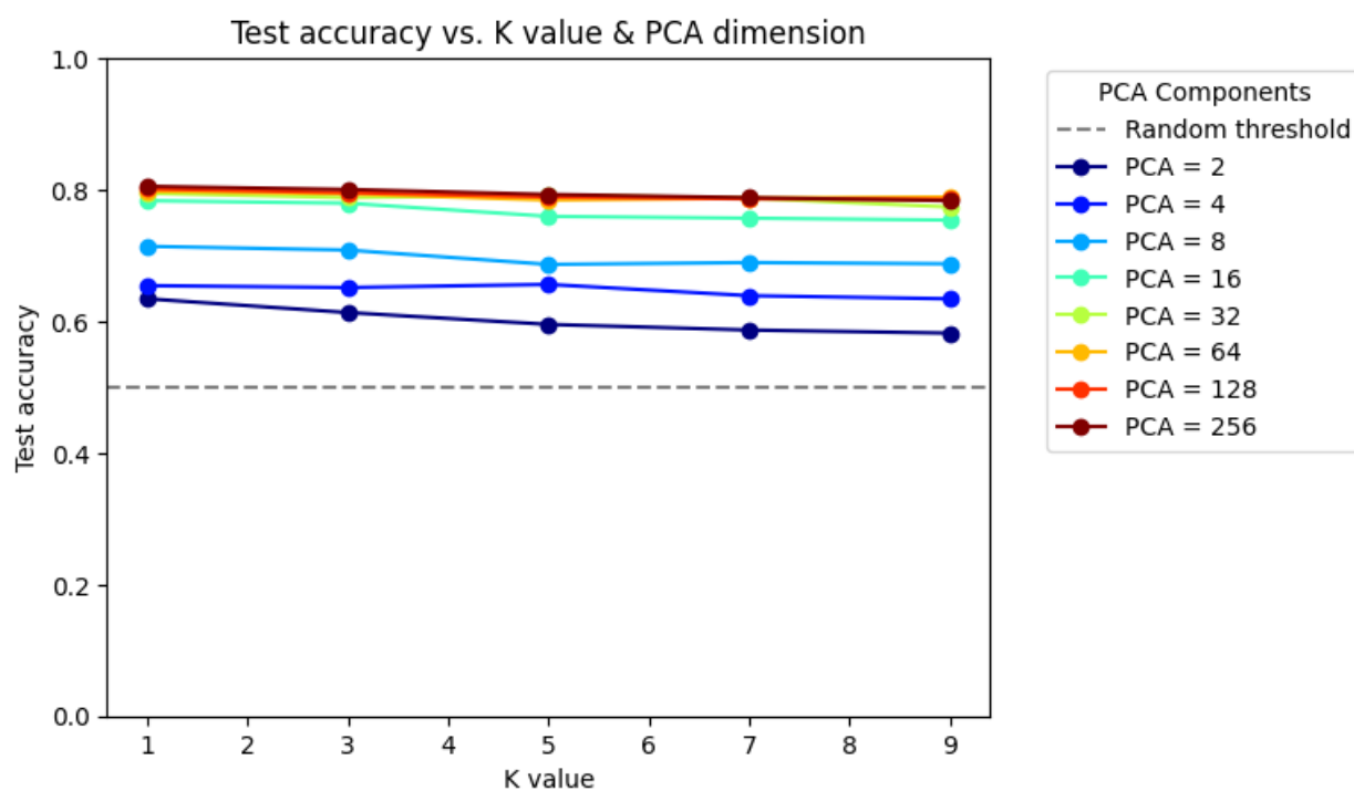
Figure 38: KNN experiment Dataset A dataset A, 1 run, CPU
