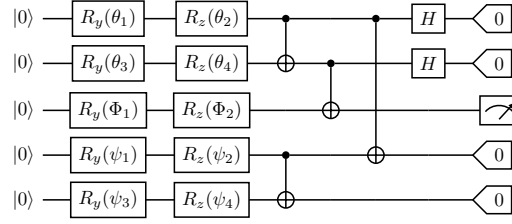
Figure 2: Pre-Alpha 1 variational quantum circuit for the sentence “John likes Mary”
