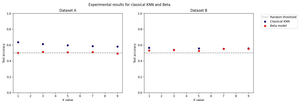
Figure 28: Classical KNN vs Beta 1, dataset A&B
