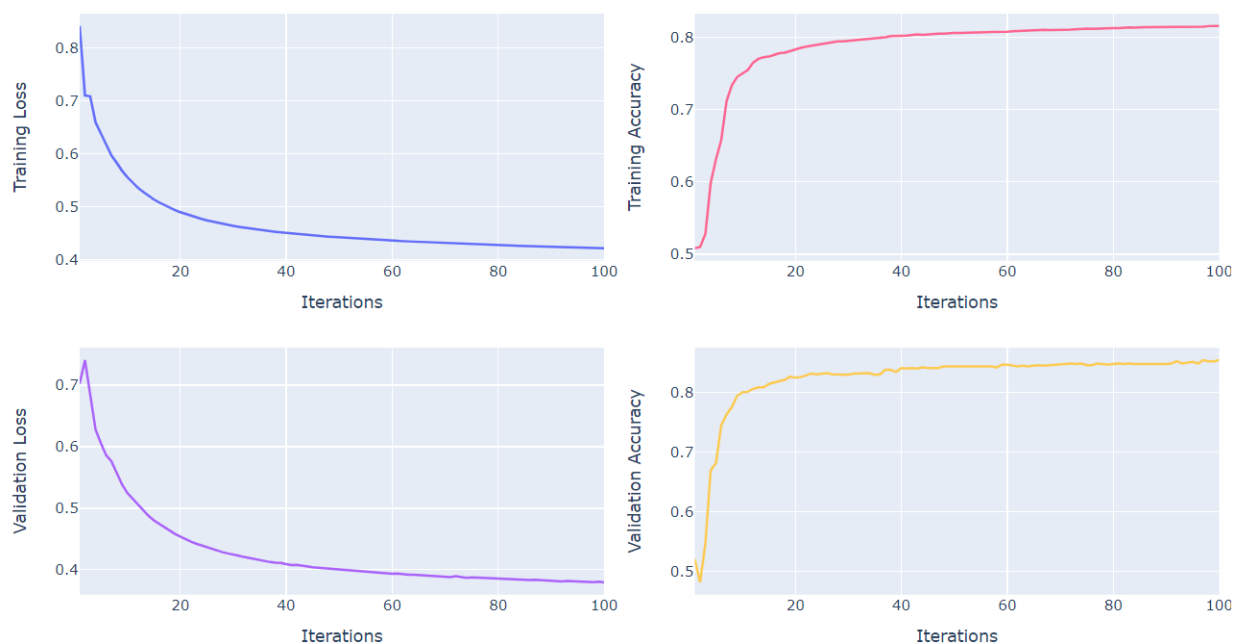
Figure 31: Shallow feed-forward neural network with BERT sentence embeddings
